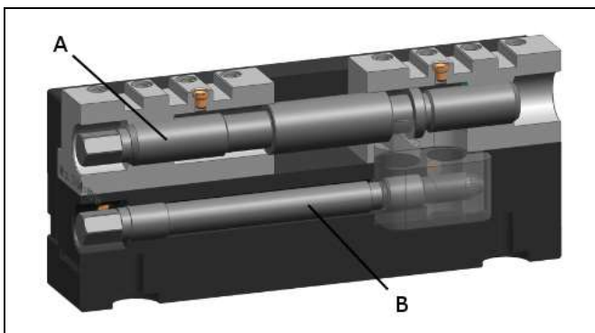
Fig. 1: Spindle drive
